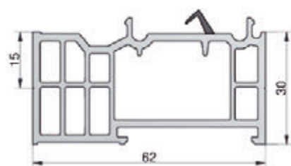
GG-TSUK6230 U_m = 1,3 \text{ W}/(\text{m}^2 \cdot \text{K})
