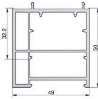
GG-TSUK5049-S U_m = 1,8 \text{ W}/(\text{m}^2 \cdot \text{K})
