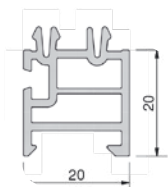
GG-TSUK2020 U_m = 2,6 \text{ W}/(\text{m}^2 \cdot \text{K})
