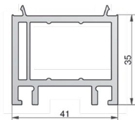
GG-TSUK4135 U_m = 1,9 \text{ W}/(\text{m}^2 \cdot \text{K})
