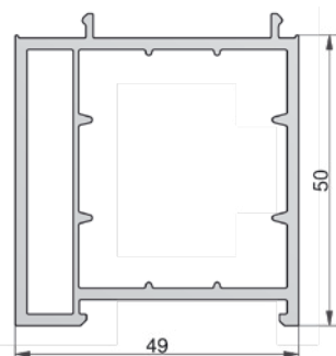
GG-TSUK5049 U_m = 1,8 \text{ W}/(\text{m}^2 \cdot \text{K})
