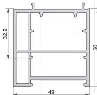
GG-SUK5049-Steg U_m = 1,8 \text{ W}/(\text{m}^2 \cdot \text{K})
